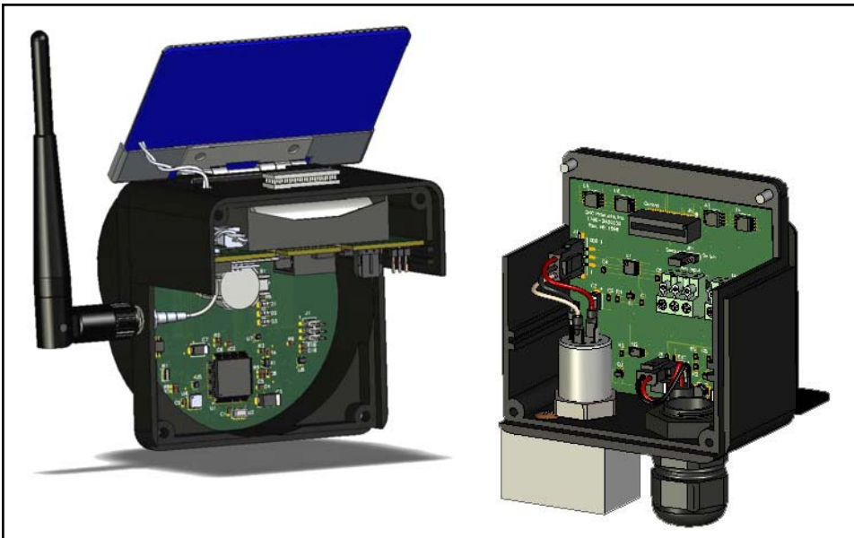
P/N 9203-2031061. AeroMate front cover assembly and sensor module shown disassembled. Front cover assembly, shown with wireless installed, is easily removed for sensor maintenance.
